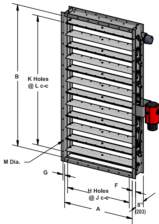
TFD80 shown with optional bolt holes and with factory supplied and mounted pneumatic actuator and proximity switch.
